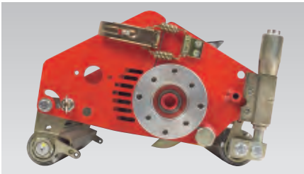
BPS Blade Protection System protects blade tips during storage
